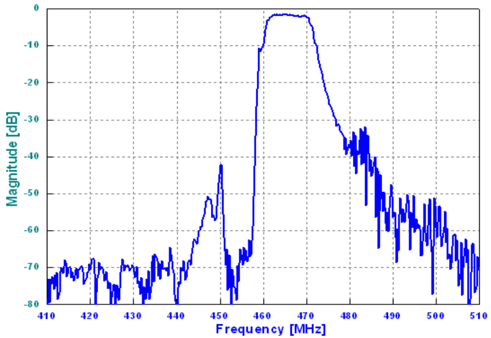
Frequency Response
